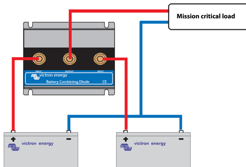
System with two batteries
